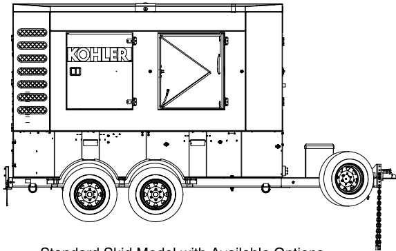
Standard Skid Model with Available Options
